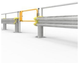
Ball-Fence with W-Beam
